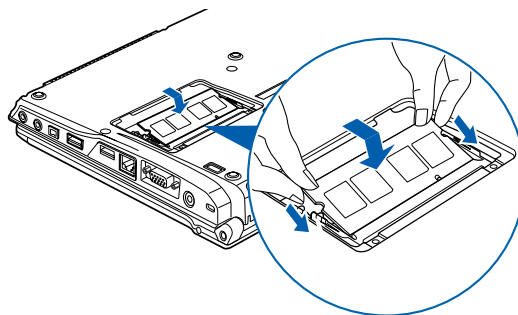
Figure 21. Inserting a Memory Module
