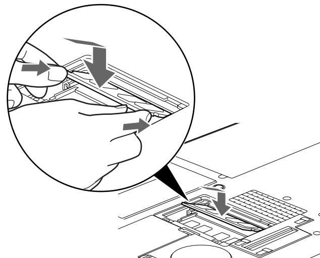
Figure 35. Installing a Second Memory Module
