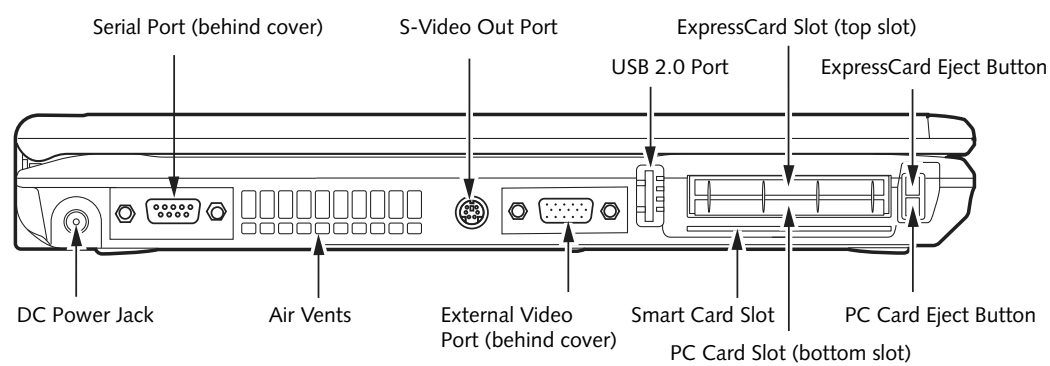
Figure 2-4. LifeBook notebook left-side panel
