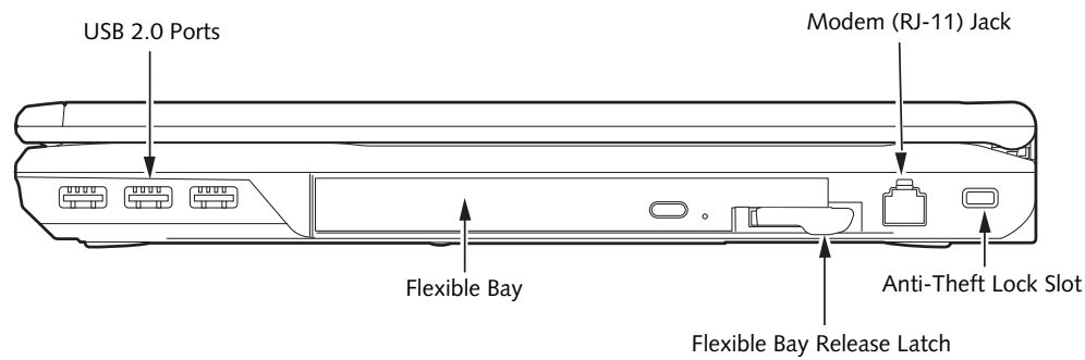
Figure 2-5. LifeBook notebook right-side panel
