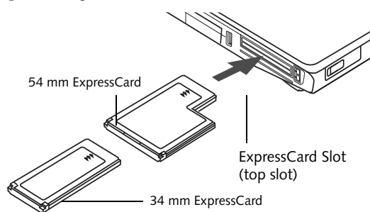
Figure 4-7. Inserting/Removing ExpressCards
