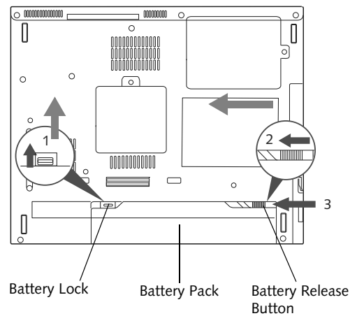
Figure 4-1. Removing a Battery
