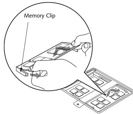
Figure 4-11. Removing a Memory Upgrade Module
