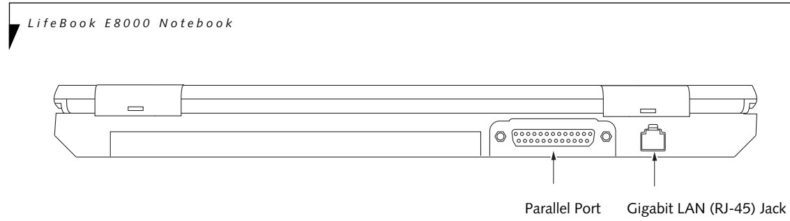
Figure 2-6. LifeBook notebook back panel
