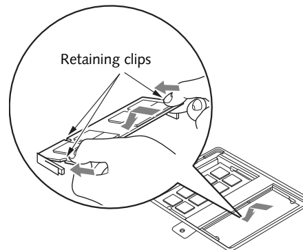
Figure 4-10. Installing a Second Memory Module
