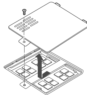
Figure 4-9. Opening the Memory Upgrade Compartment
