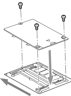
Figure 4-4. Replacing the Memory Compartment Cover
