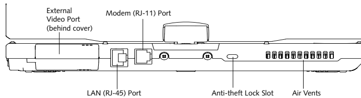
Figure 2-7. LifeBook P Series notebook/Tablet PC rear panel
