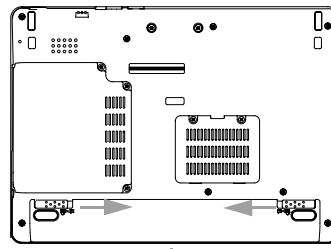
Figure 4-1. Removing the Battery
