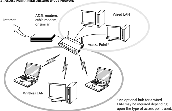
Figure A-2. Access Point (Infrastructure) Mode Network
