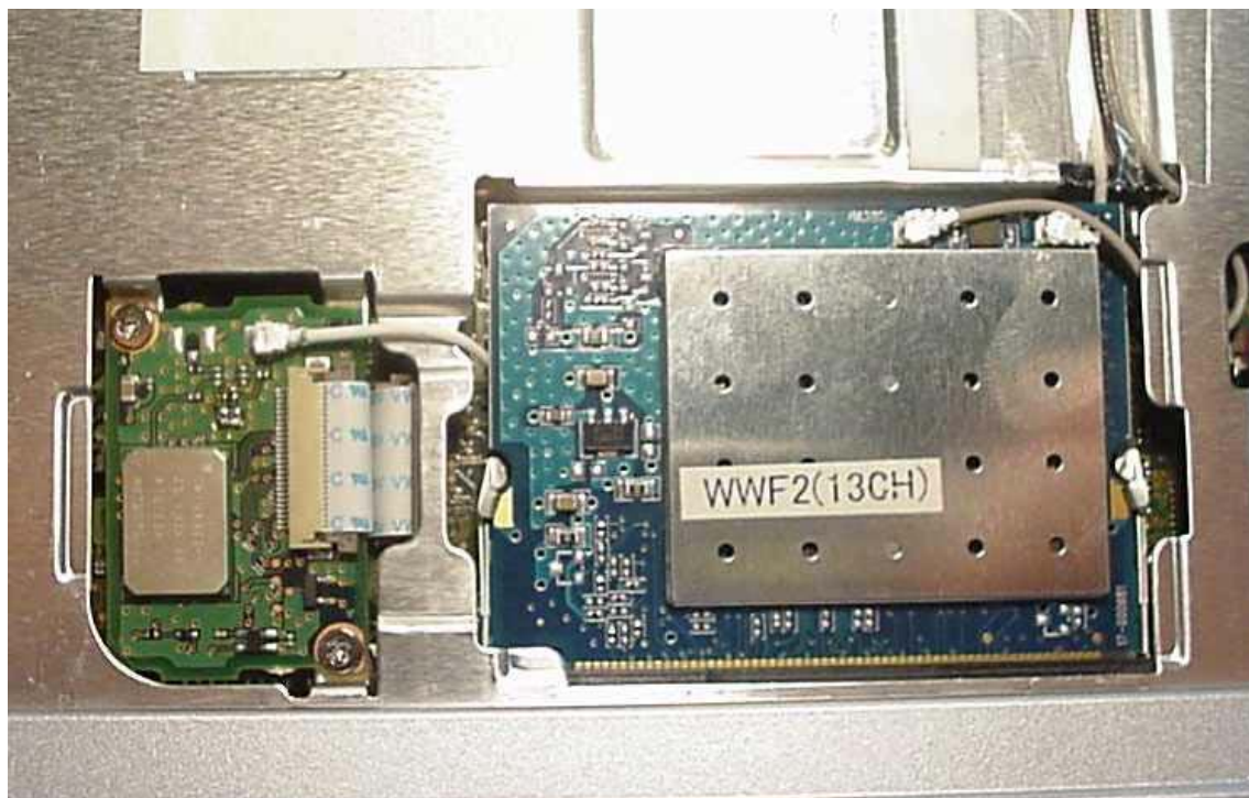
WLL4070 inside the Fujitsu Tablet Computer
