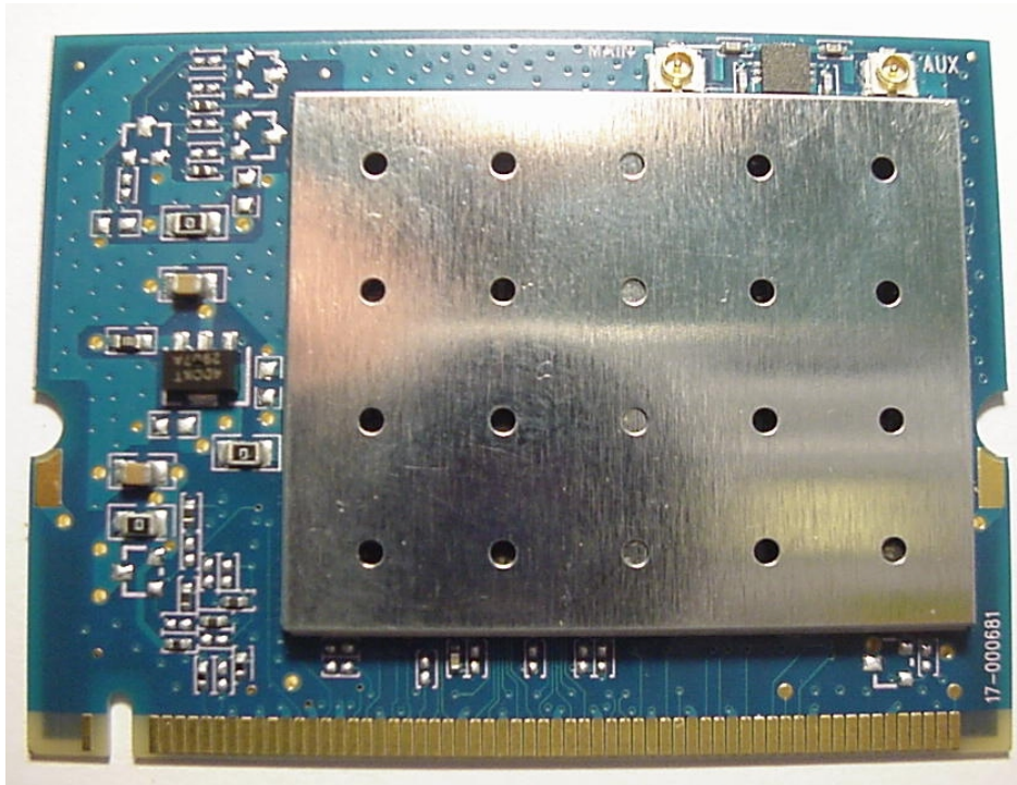
Model: WLL4070 – WLAN Module Front
