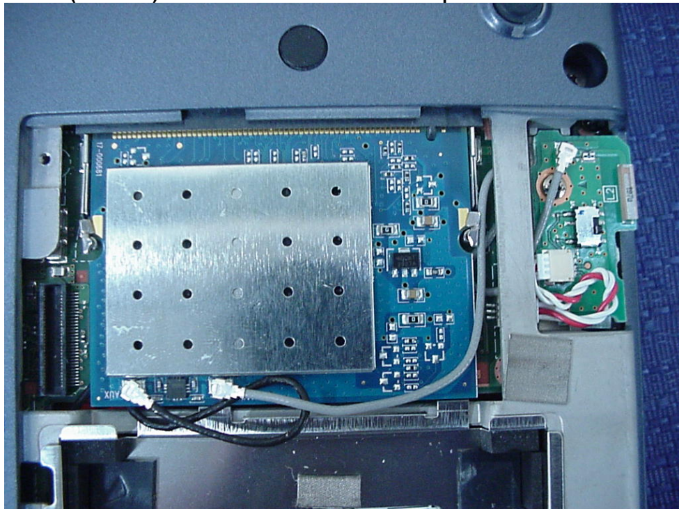
Atheros (WLL4070) WLAN and Antenna Location – exploded view
