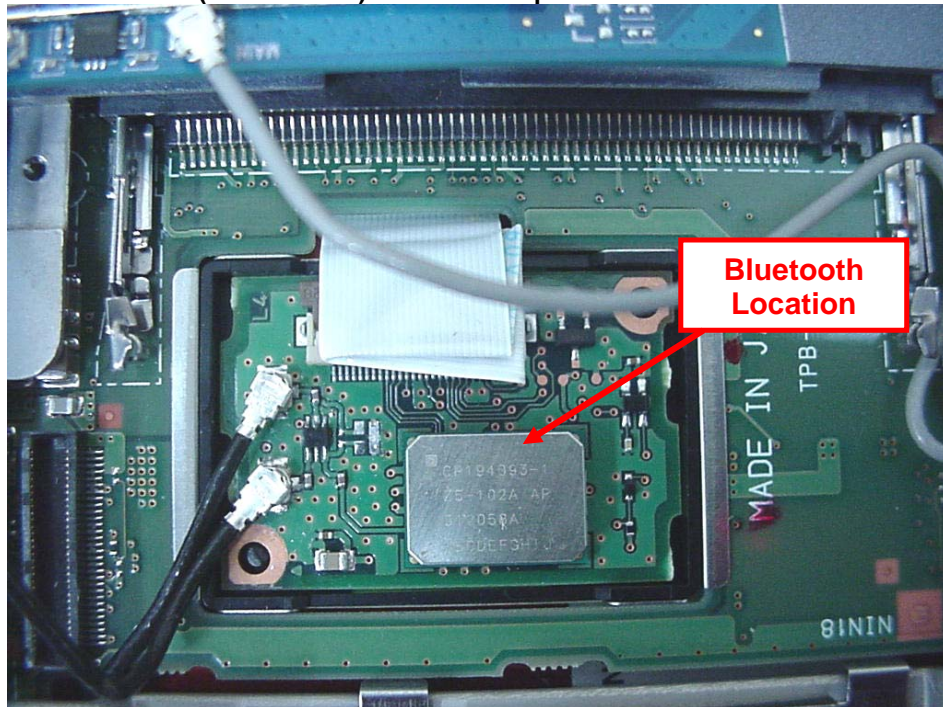
Bluetooth (UGXZ5-102A) Location – exploded view
