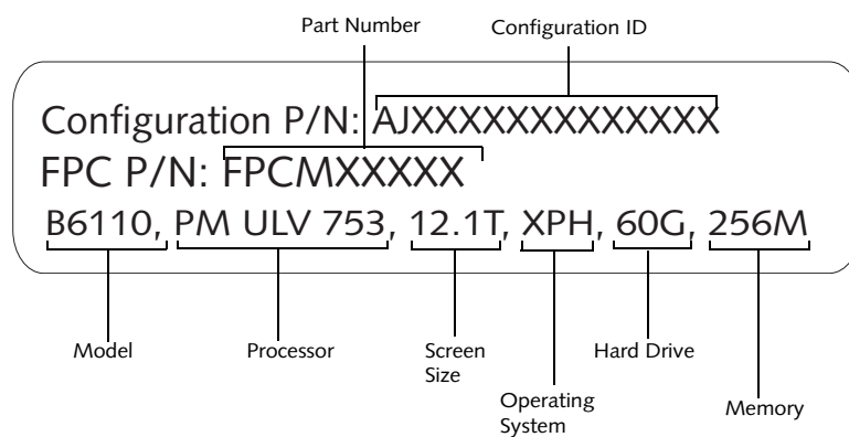
Figure 7-1. Configuration Label
