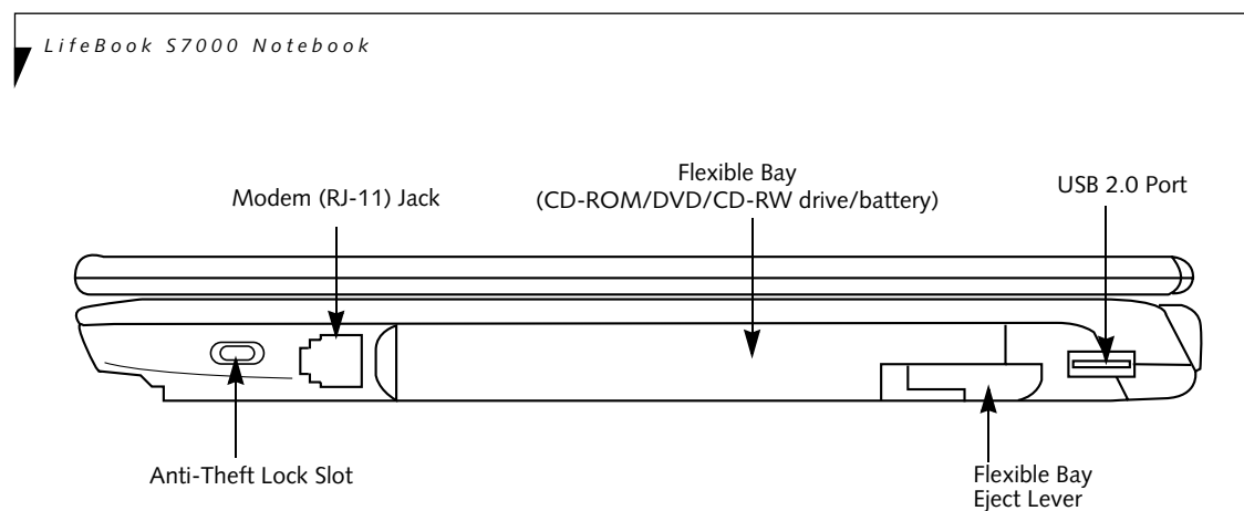
Figure 2-5. LifeBook notebook right-side panel
