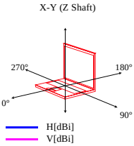
The Measurement Result Antenna Radiation Pattern X-Y
