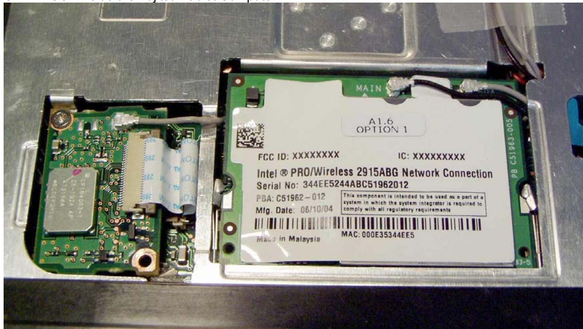
CALEXICO2 inside the Fujitsu Tablet Computer
