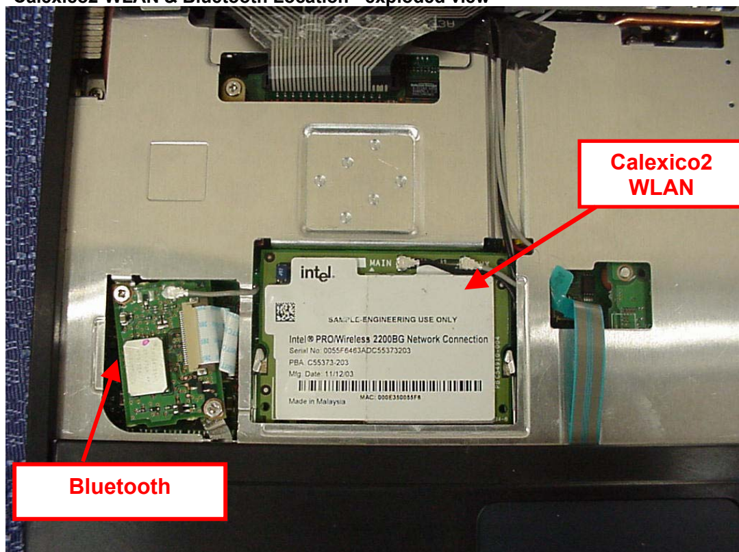
Calexico2 WLAN & Bluetooth Location - exploded view
