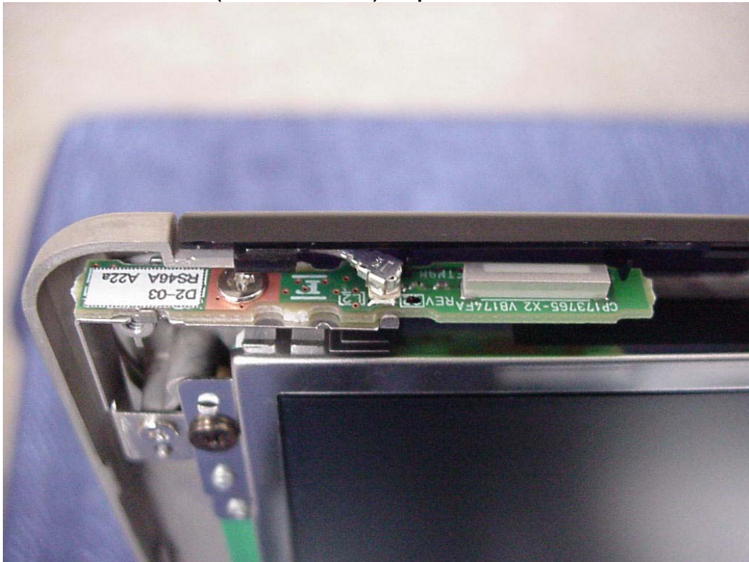
Left Antenna Location (Calexico2 WLAN) - exploded view
