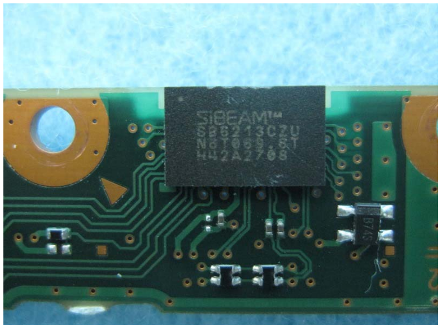
60G Module and antenna Model No.: SB6213
