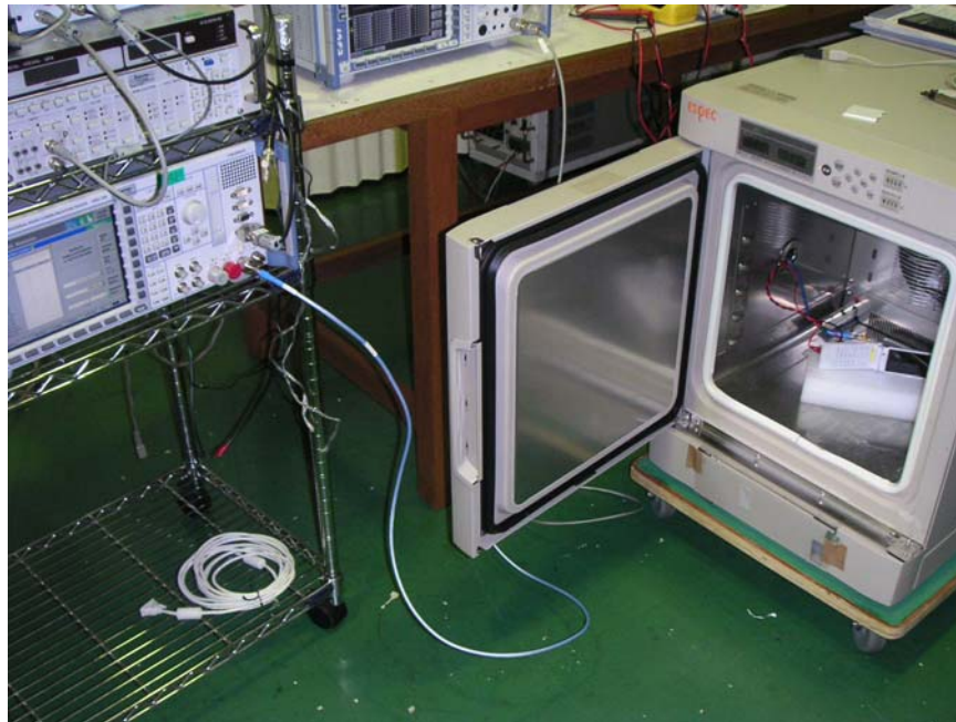
Temperature test (Frequency Stability)
