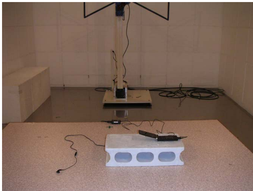
Radiated emission
