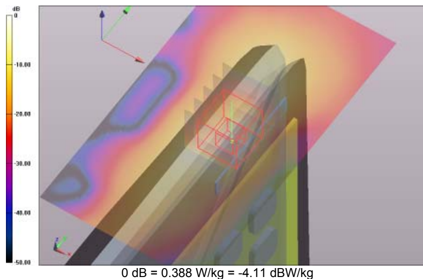
SAR Measurement Plot 172
