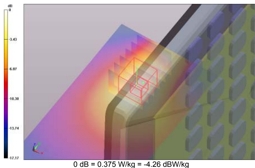
SAR Measurement Plot 98
