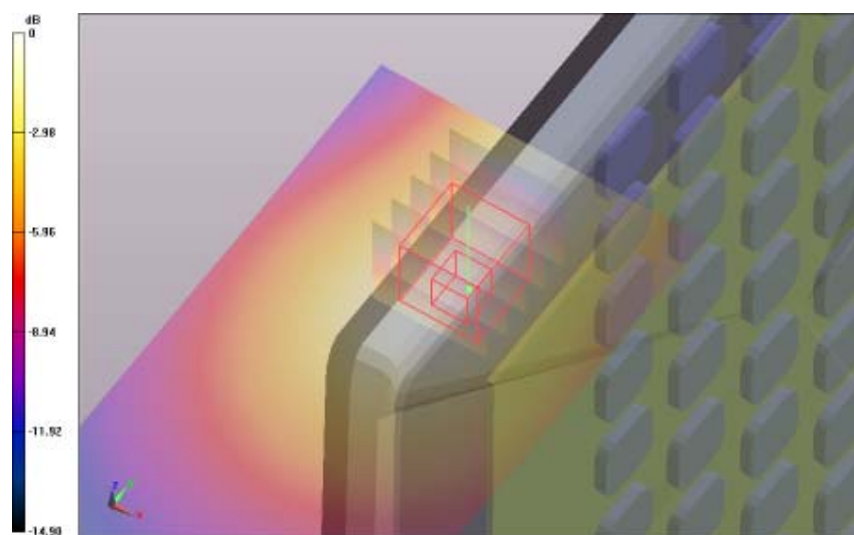
SAR Measurement Plot 121
