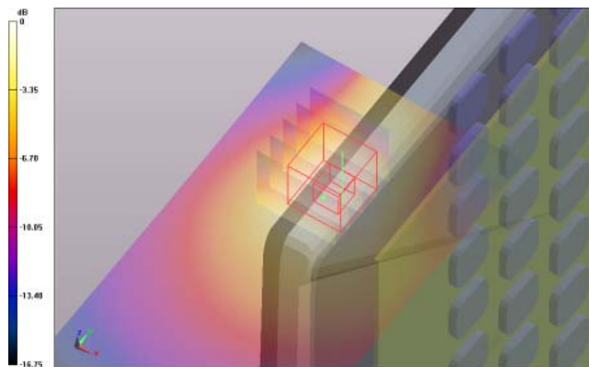
SAR Measurement Plot 157
