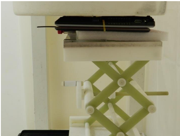
Bottom Face, Antenna Swivel 90 Test Separation 0 cm
