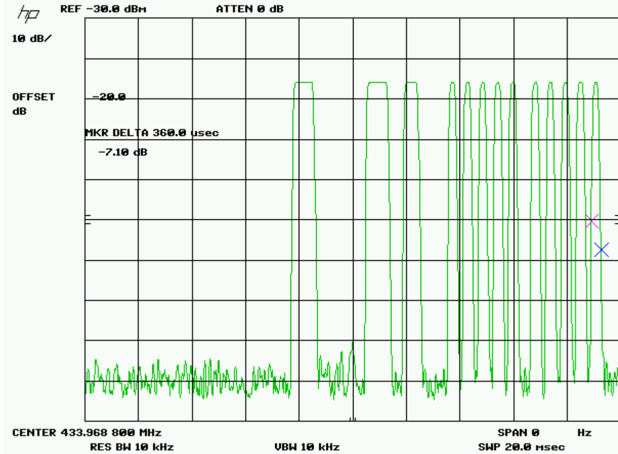
DUTY CYCLE PLOT – SHORT PULSES
