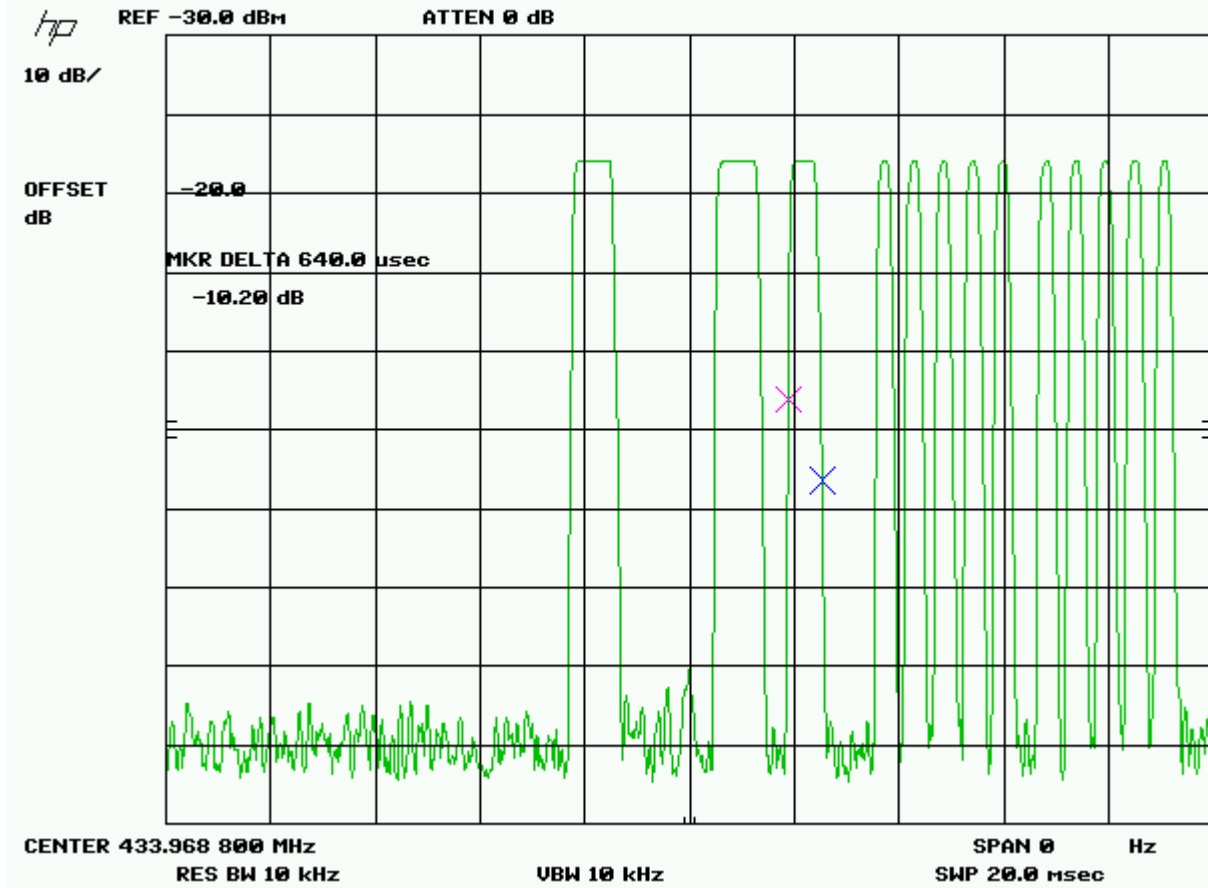
DUTY CYCLE PLOT - MEDIUM PULSES
