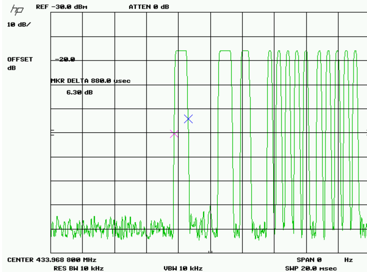
DUTY CYCLE PLOT - LONG PULSES
