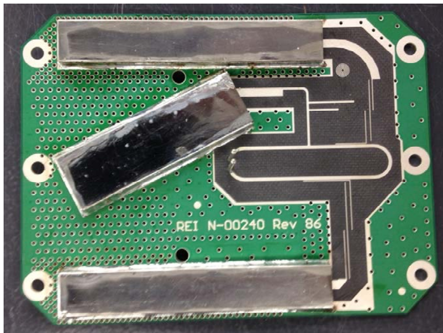
N-00240 Multiplexer Board – Side A (with shields):
