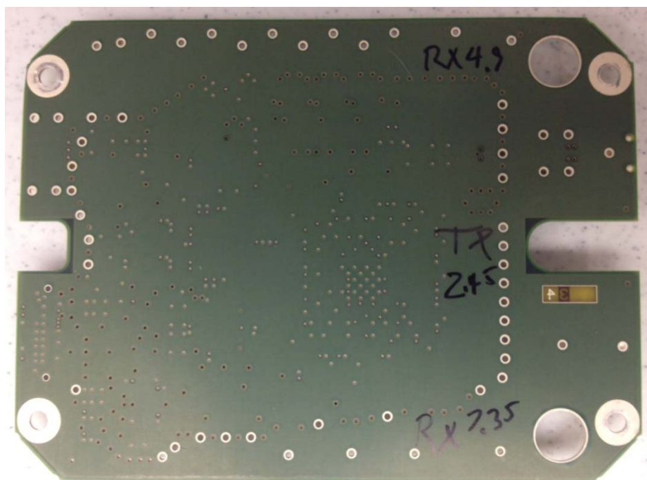
N-00260 Digital Board – Side B:
