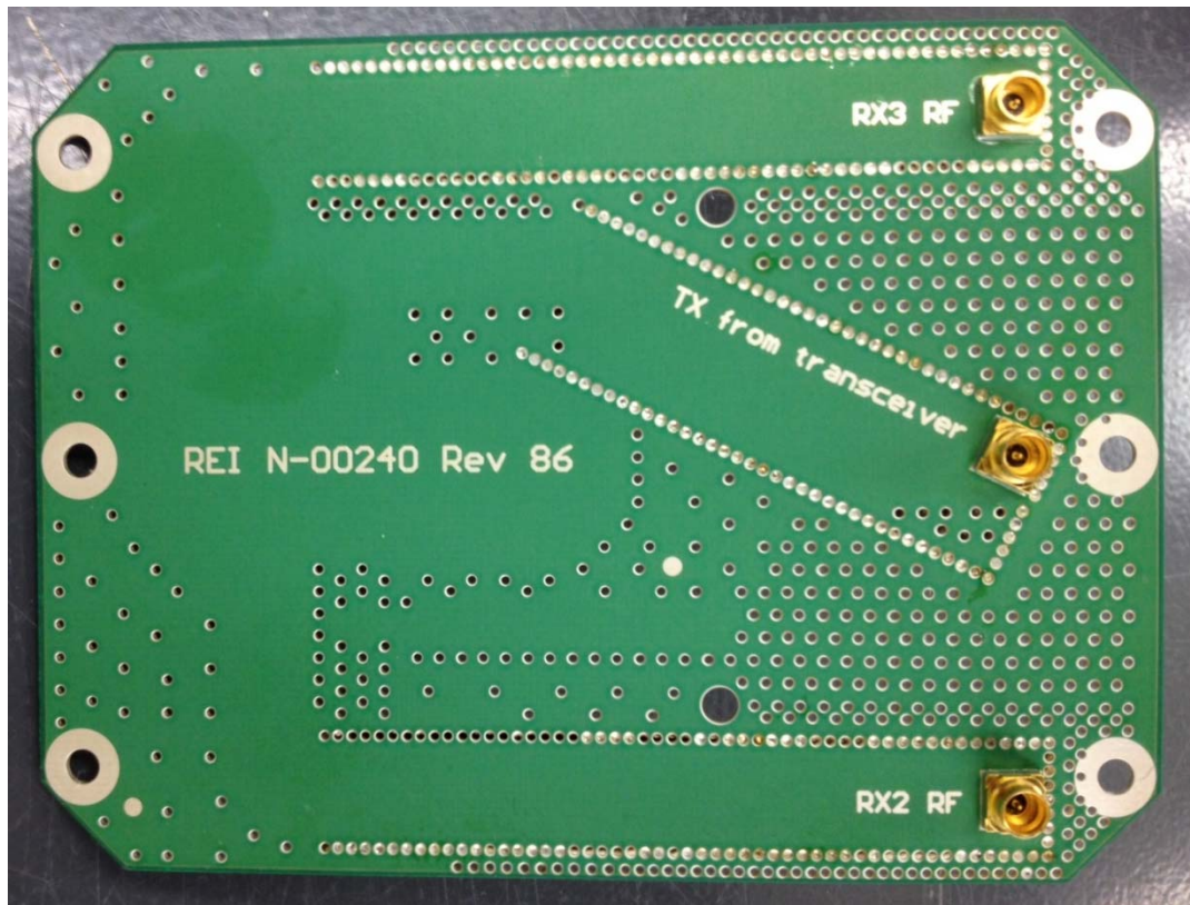
N-00240 Multiplexer Board – Side B:
