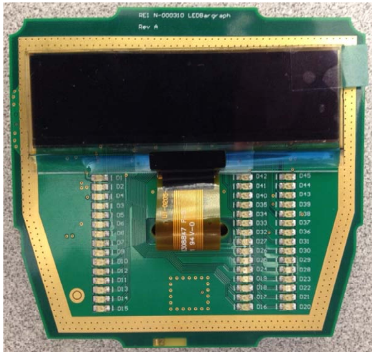
N-00310 LED Bargraph Board – Side B:
