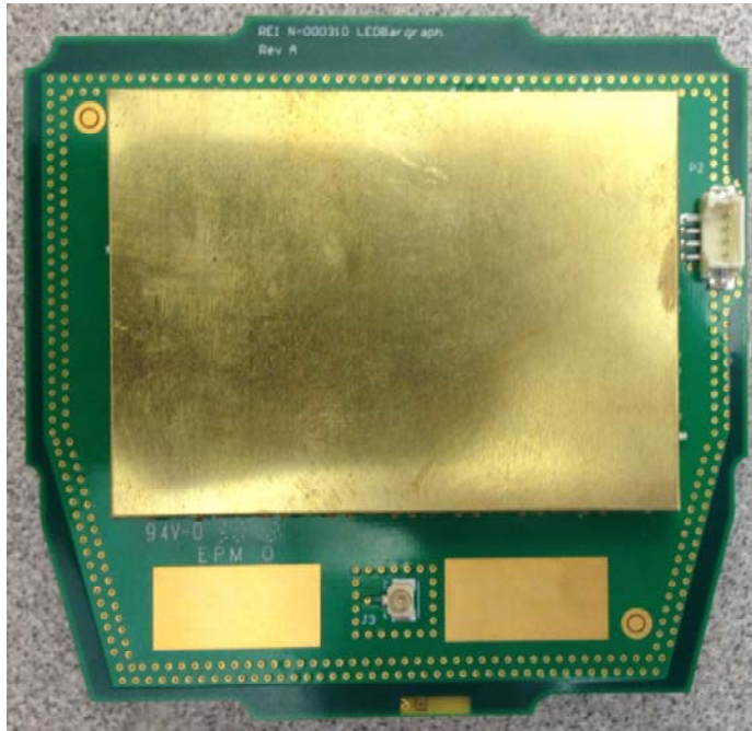
N-00310 LED Bargraph Board – Side A (with shields):
