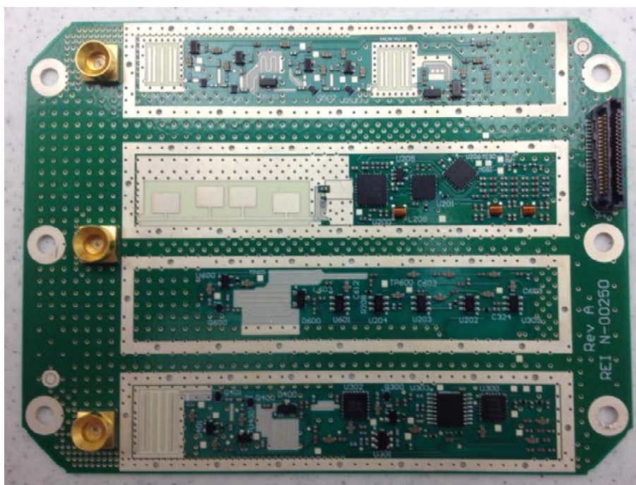
N-00250 RF Board – Side A (without shields)
