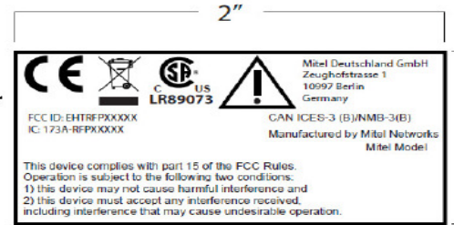
FCC Label
