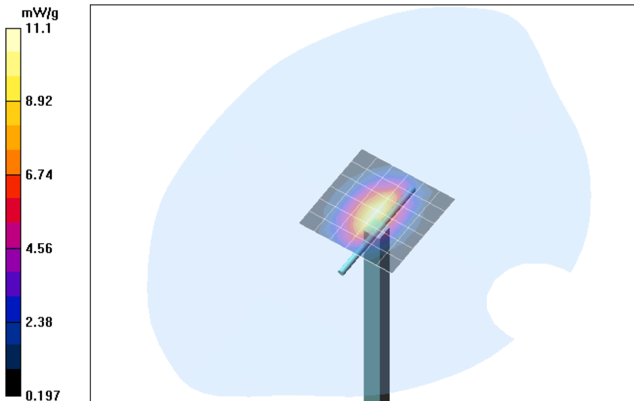
Fig. 8: Validation measurement 1900 MHz Head (May 15, 2007), coarse grid. Ambient Temperature: 21.8° C, Liquid Temperature: 21.0° C.
