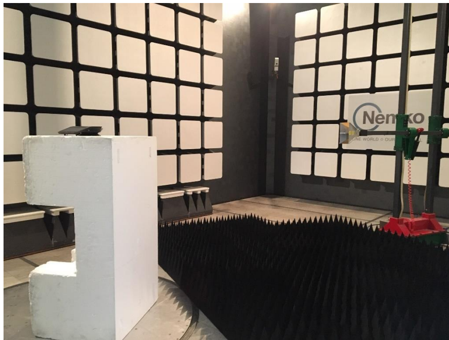
Figure 1.1-3: Radiated emissions setup photo – above 1 GHz
