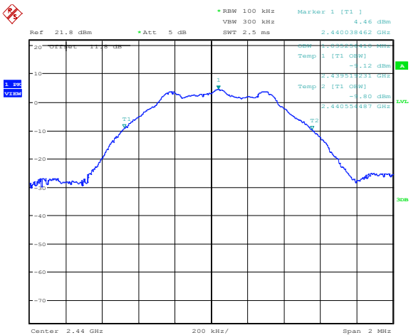
Figure 8.5-5: 99% occupied bandwidth – Mid channel
