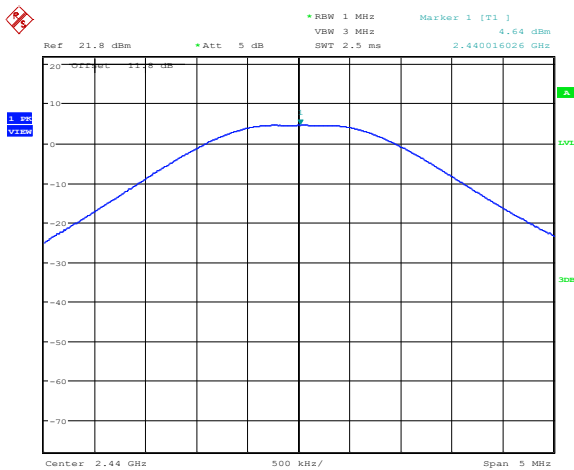
Figure 8.6-2: Output power on mid channel
