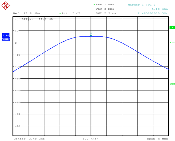
Figure 8.6-3: Output power on high channel
