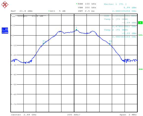
Figure 8.5-6: 99% occupied bandwidth – High channel
