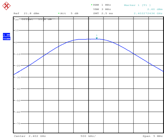
Figure 8.6-1: Output power on low channel
