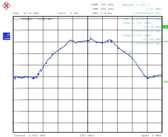
Figure 8.5-4: 99% occupied bandwidth – Low channel
