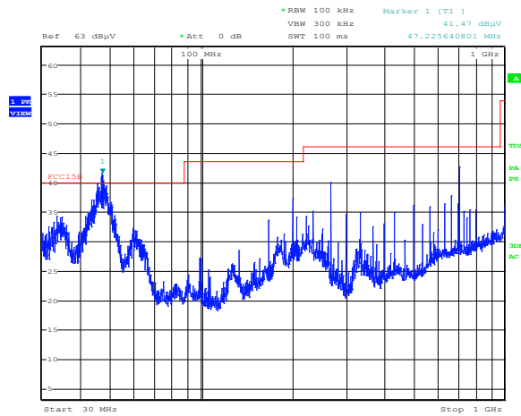
Figure 8.6-40: Radiated spurious emissions for BT, high channel, 30 to 1000 MHz
