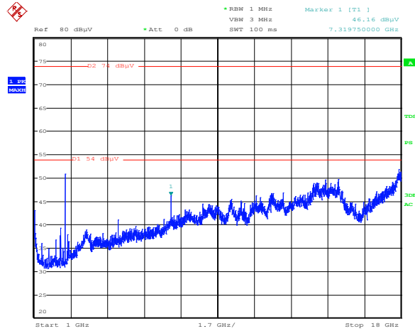
Figure 8.6-61: Radiated spurious emissions for BLE, mid channel, 1 to 18 GHz
