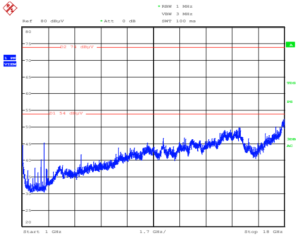
Figure 8.6-60: Radiated spurious emissions for BLE, low channel, 1 to 18 GHz
