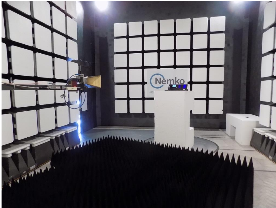
Figure 1-4: Radiated emissions setup photo – above 1 GHz
