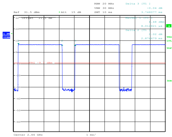
Figure 8.5-7: Pulse width for DM3
