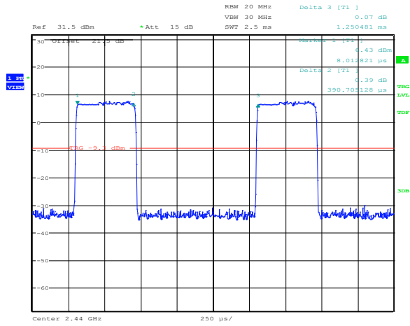
Figure 8.5-3: Pulse width for DH1
