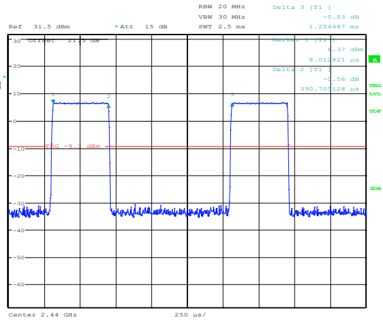
Figure 8.5-4: Pulse width for 2-DH1
