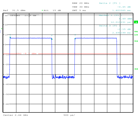
Figure 8.5-20: Pulse width for EV3
