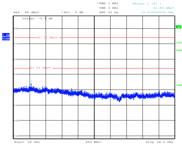
Figure 8.5-63: Radiated spurious emissions for BLE, low channel, 18 to 26.5 GHz
