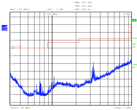
Figure 8.5-38: Radiated spurious emissions for BT, low channel, 30 to 1000 MHz
