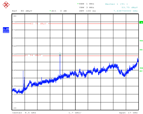
Figure 8.5-43: Radiated spurious emissions for BT, high channel, 1 to 18 GHz
