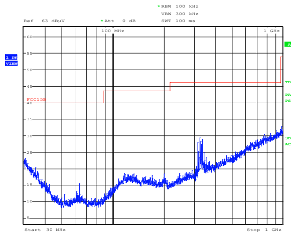
Figure 8.5-40: Radiated spurious emissions for BT, high channel, 30 to 1000 MHz
