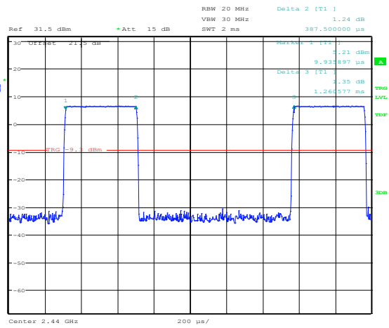
Figure 8.5-16: Pulse width for HV1
