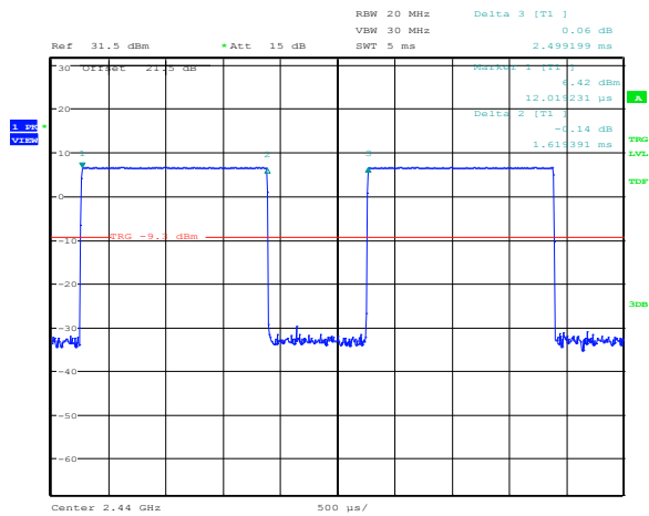
Figure 8.5-19: Pulse width for DV
