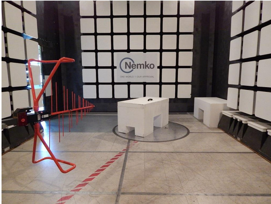
Figure 8.5-69: Radiated spurious (out-of-band) emissions setup photo – 30 to 1000 MHz
