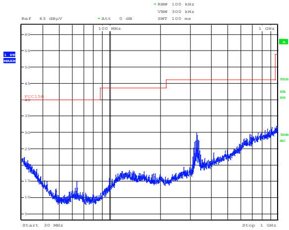
Figure 8.5-57: Radiated spurious emissions for BLE, low channel, 30 to 1000 MHz
