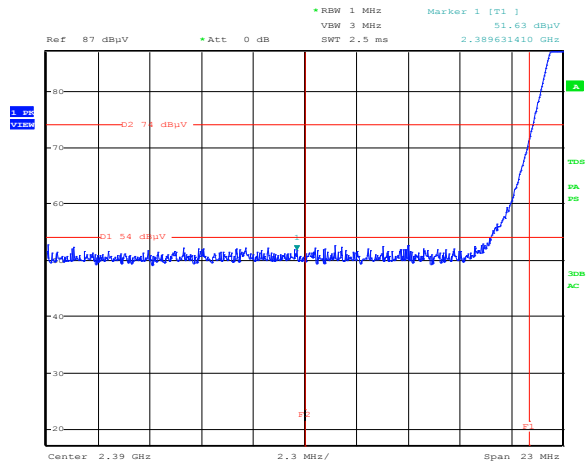
Figure 8.5-55: Radiated spurious emissions Lower band edge emission for BLE, low channel. F_2 = 2.39 GHz (end of restricted band), F_1 = 2.4 GHz
