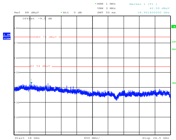
Figure 8.5-46: Radiated spurious emissions for BT, high channel, 18 to 26.5 GHz
