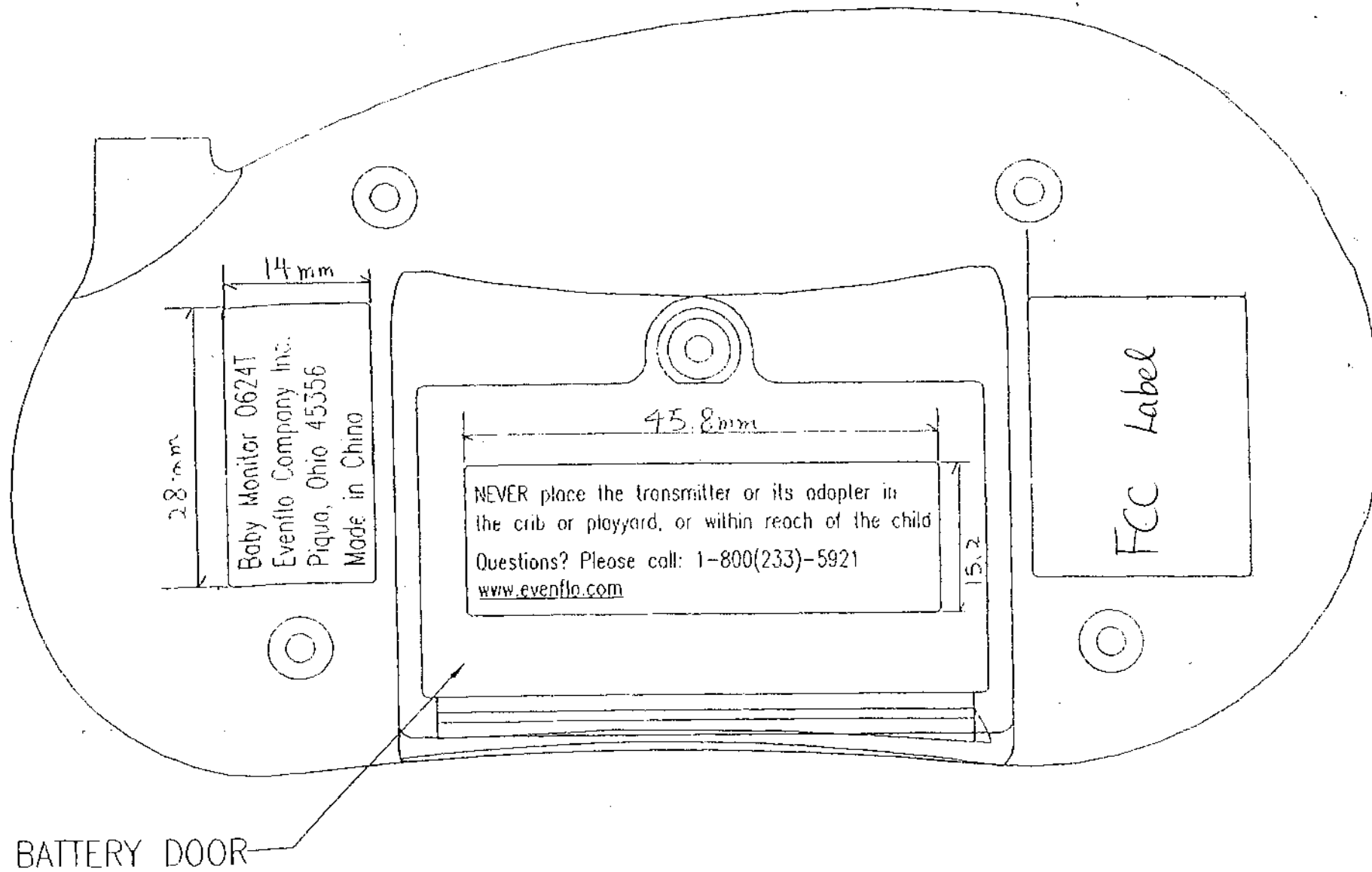
MODEL 0624 TX FCC ENGRAVING DRAWING
