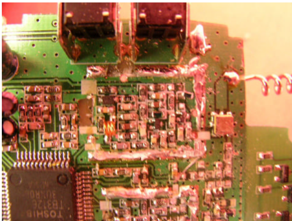
Base Oscillator PCB comp side (View 1)
