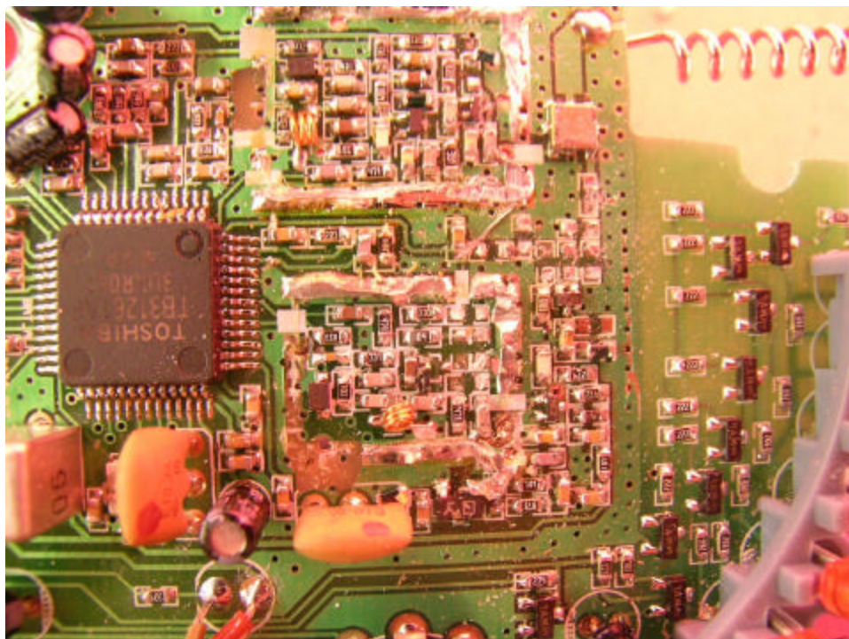
Base Oscillator PCB comp side (View 2)
