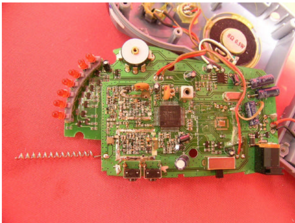
Base Main PCB comp side (View 2)
