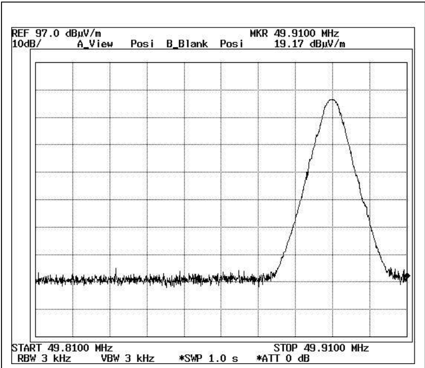
Un-modulated Carrier Channel B
