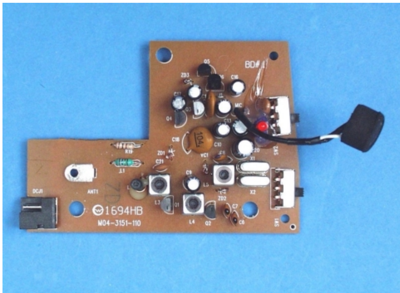
Circuit Board – Component Side
