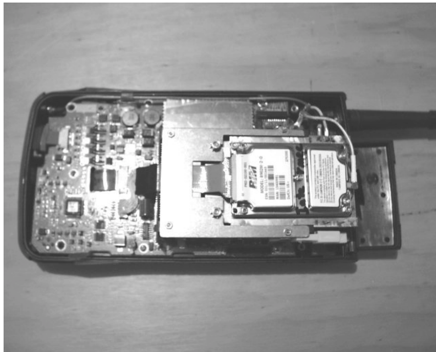
Photo 1: Shows a close-up view of the RIM902 radio installed within the 6100 tablet computer.
