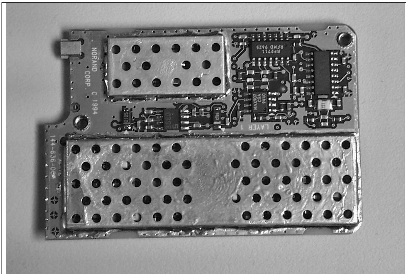
Front view of radio PCB
