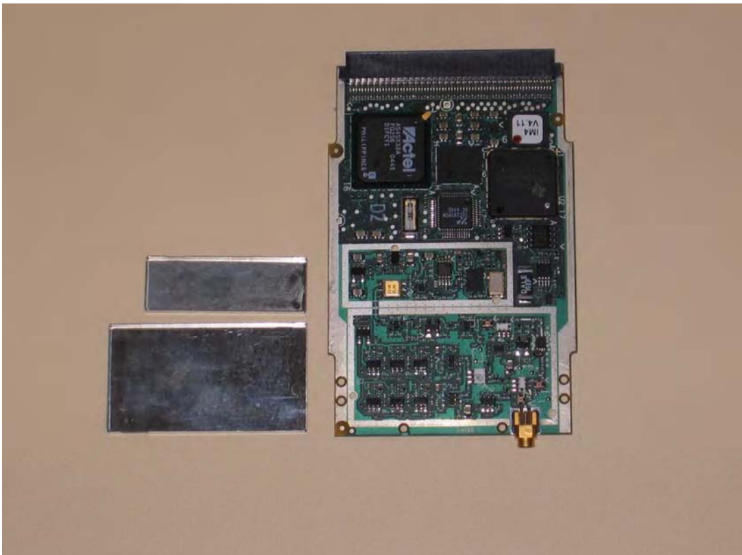
Top of IM4 PCB with Shields Removed
