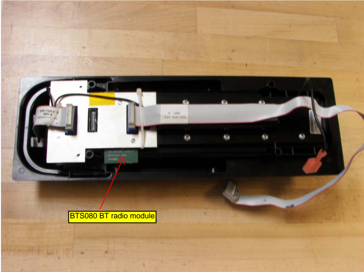
700C Terminal Holder – Bottom View
