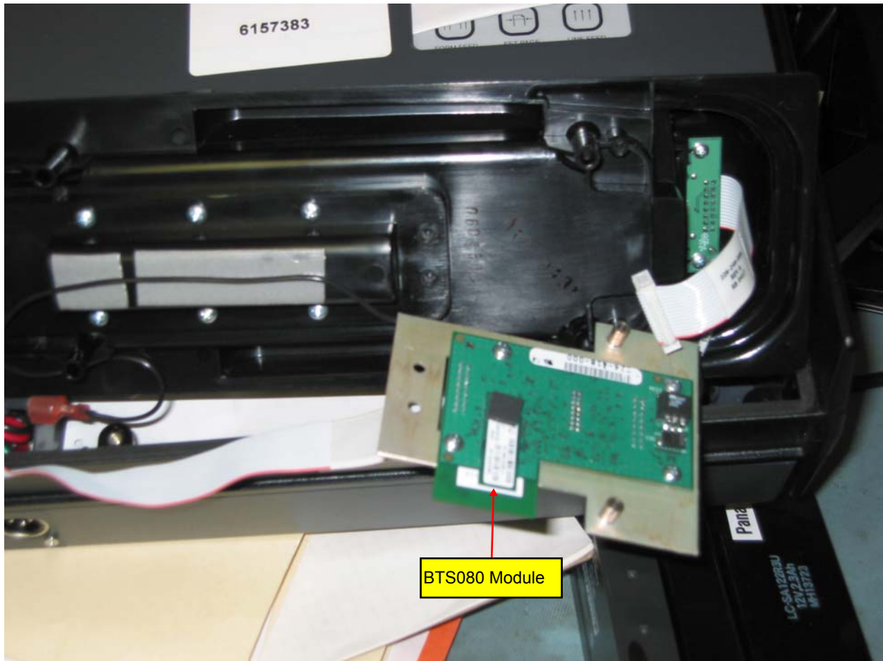
Aluminum mounting plate removed from bottom of terminal holder to show BTS080 module
