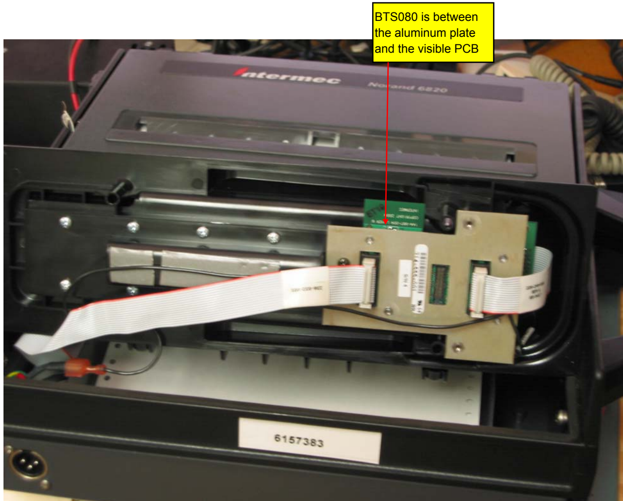
6820 Printer with 700C terminal holder unbolted and turned for viewing
