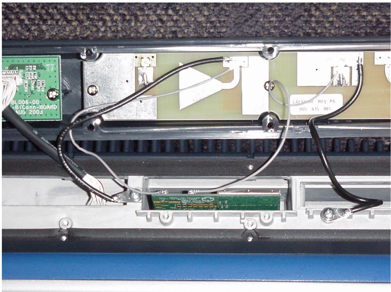
CV60 Shows 805-615-304 Antenna Board and 802abg Radio Module
