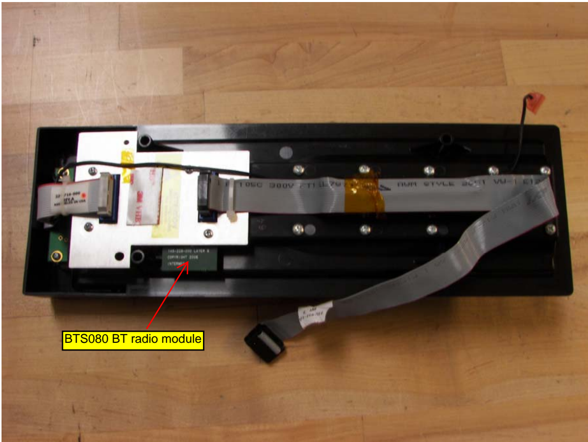
CK60 Terminal Holder – Bottom side
