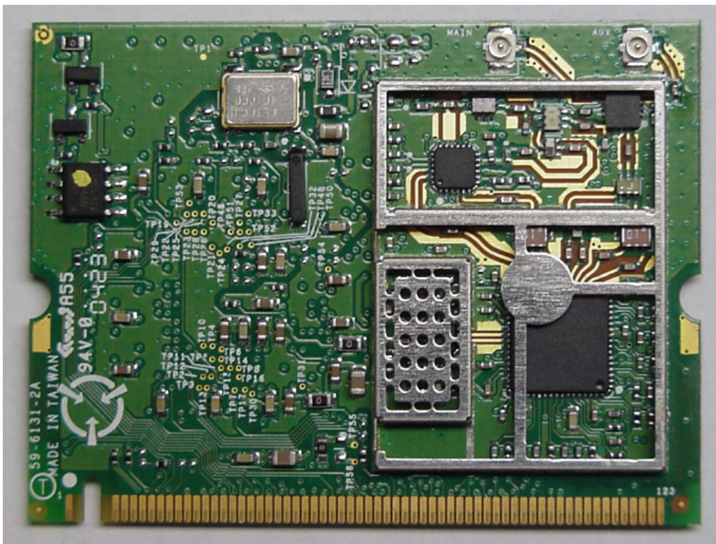
802MIAG Radio Card with Shield Removed
