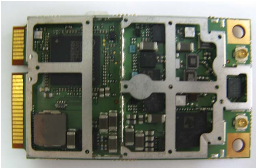
Picture 2: the back view of the sample without shielding cover
