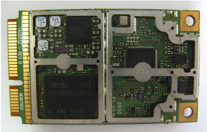
Picture 1: the front view of the sample without shielding cover
