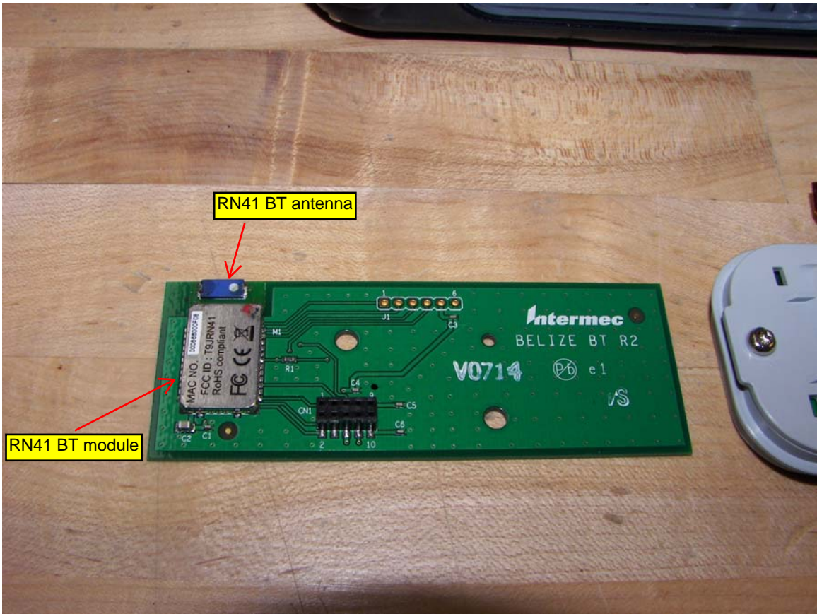
Display board – close-up of RN41 BT module mounted on display board
