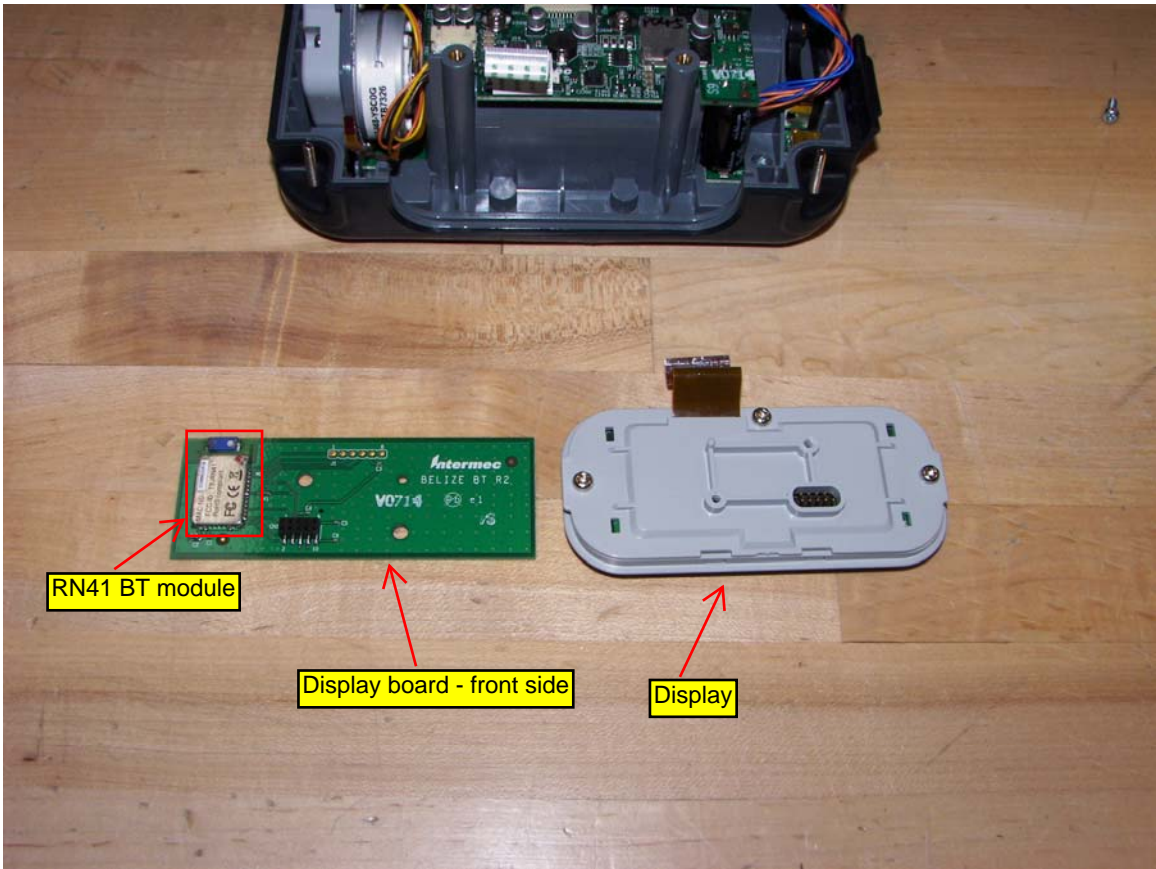
Display removed – showing display board with RN41 BT module
