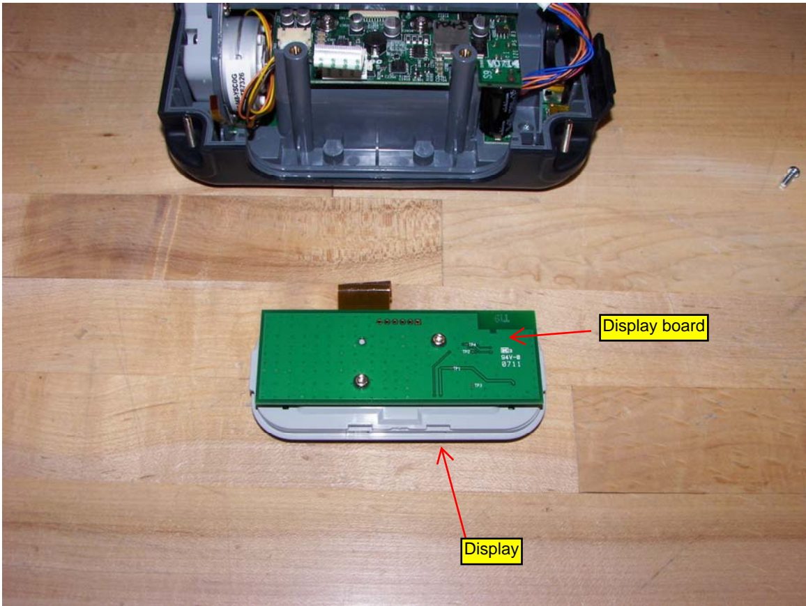
Display removed – back side of display
