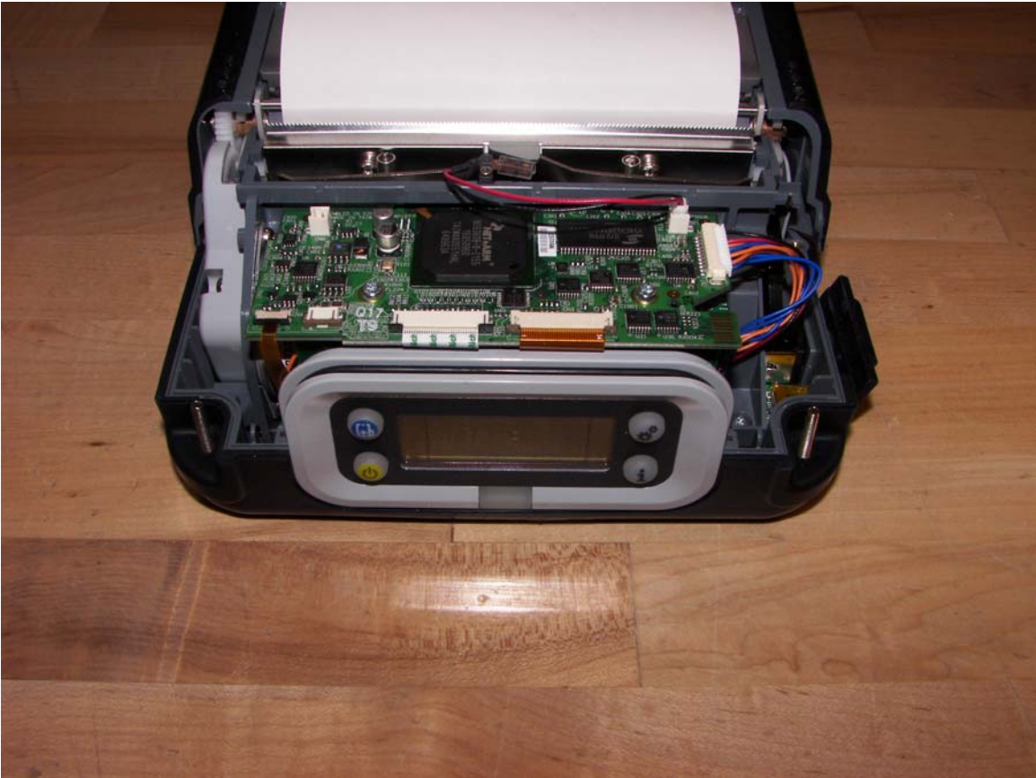
Top View: Cover removed
