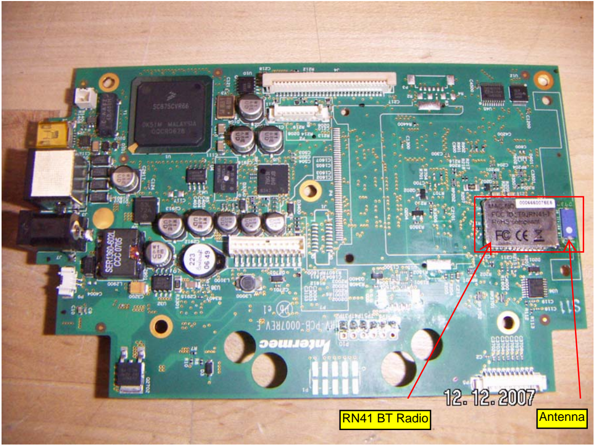
PB42 PCB – top side
