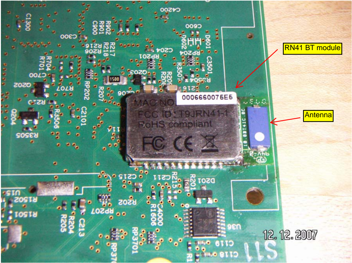
PB42 PCB – top side: RN41 BT radio module close-up
