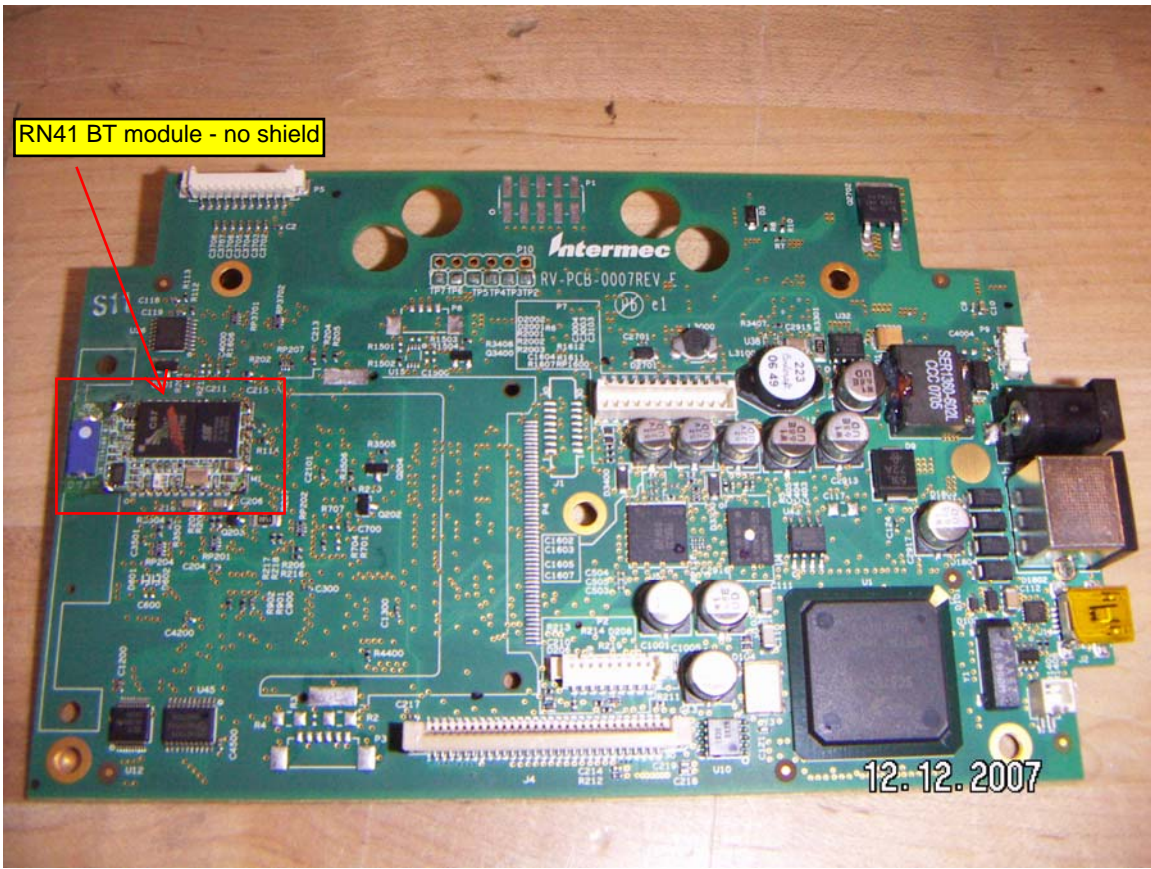
PB42 PCB – top side: RN41 shield removed
