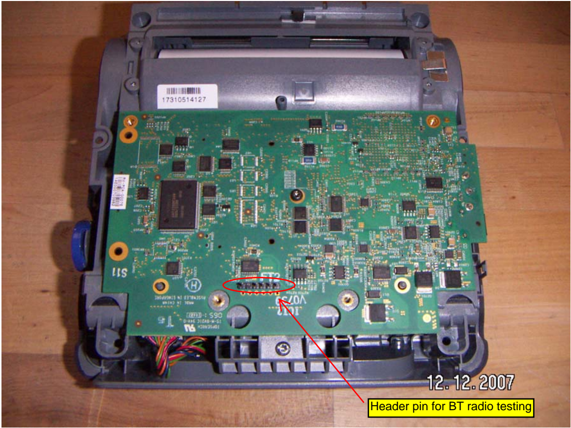
PB42 with bottom enclosure removed.
