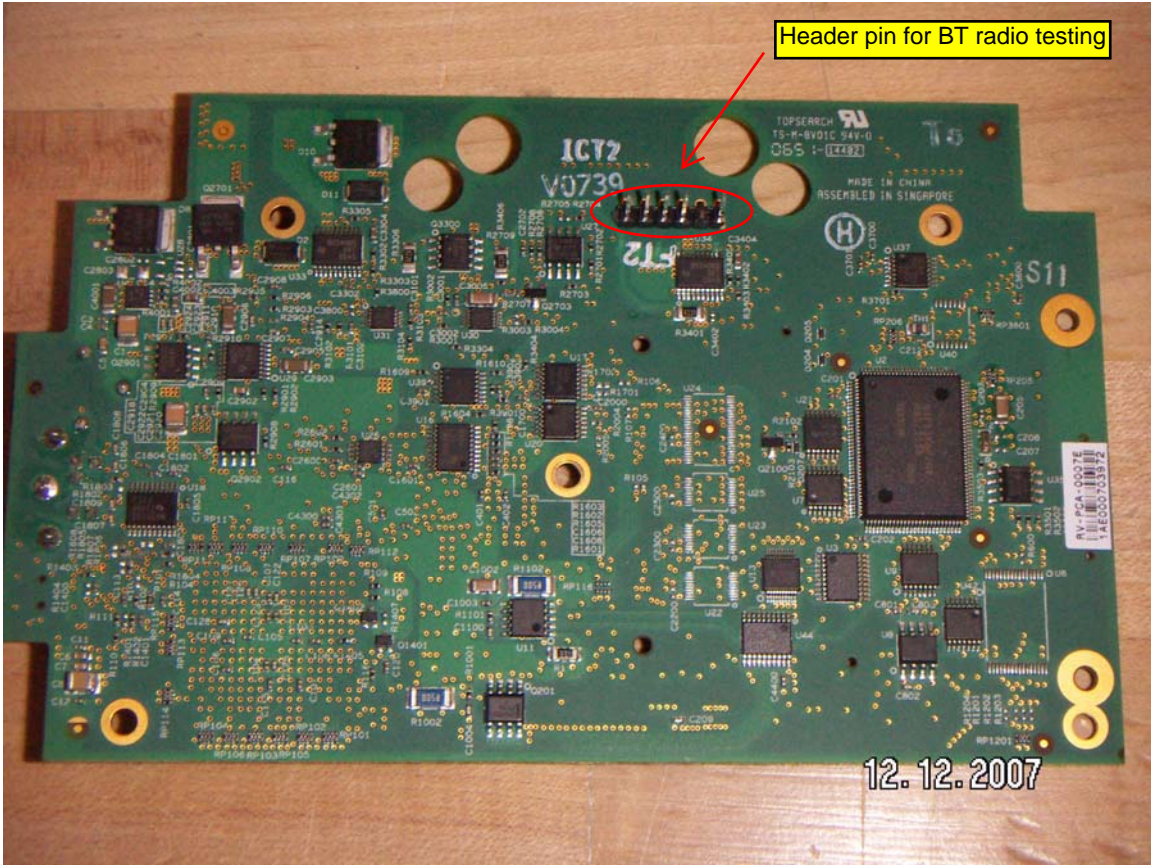
PB42 PCB removed – bottom side
