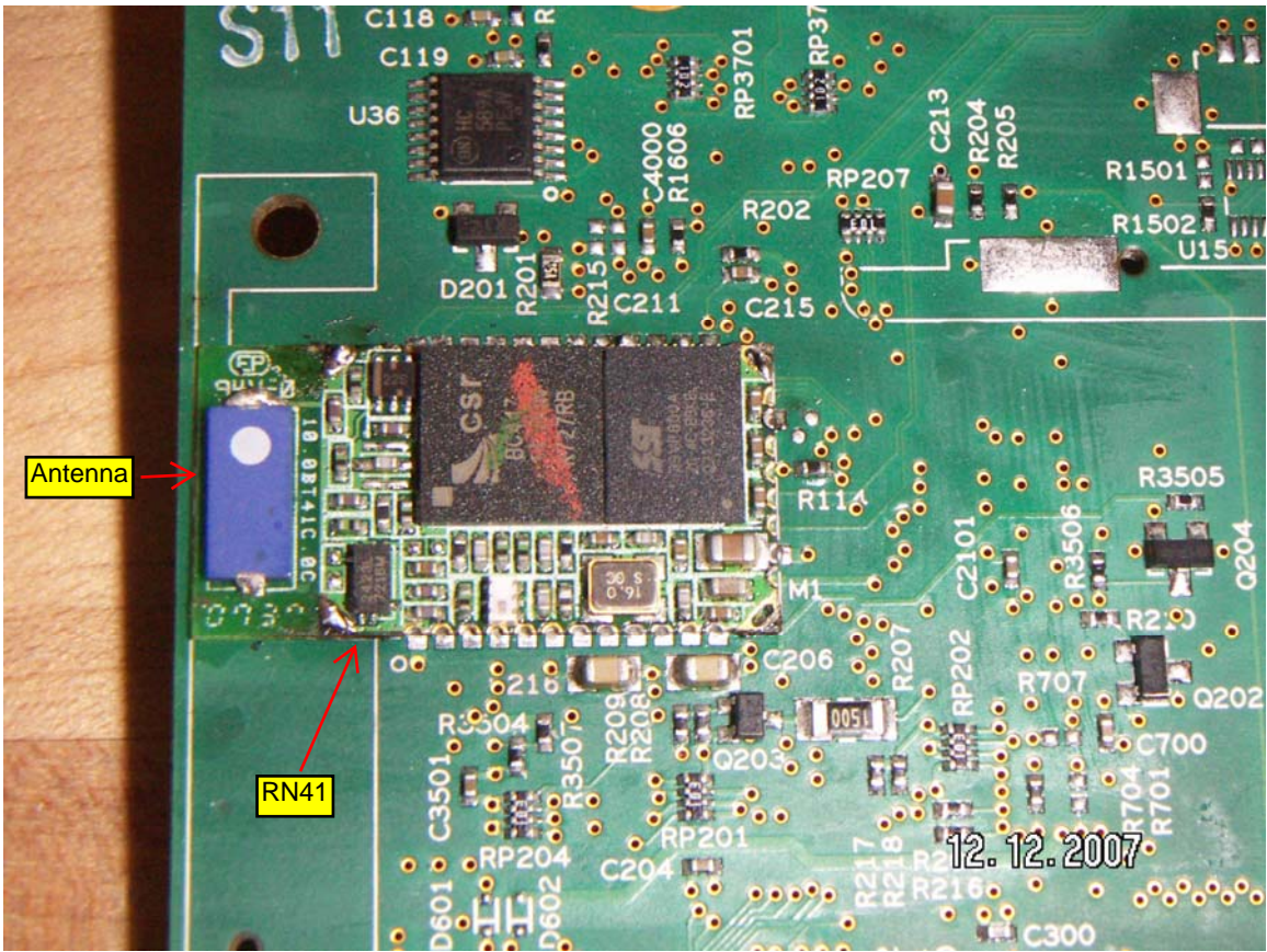
PB42 PCB – top side: RN41 shield removed close-up
