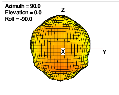
Total ERP, Front Face View
