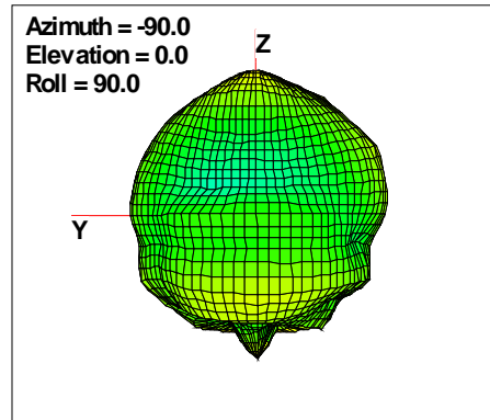
Total ERP, Back Face View
