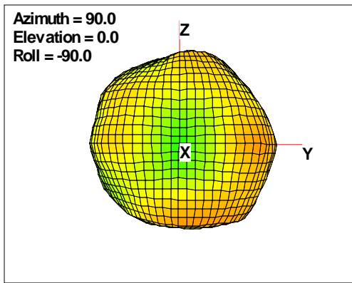
Total EIRP, Front Face View
