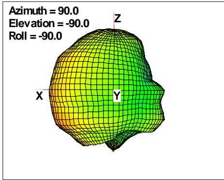
Total ERP, Right Side View
