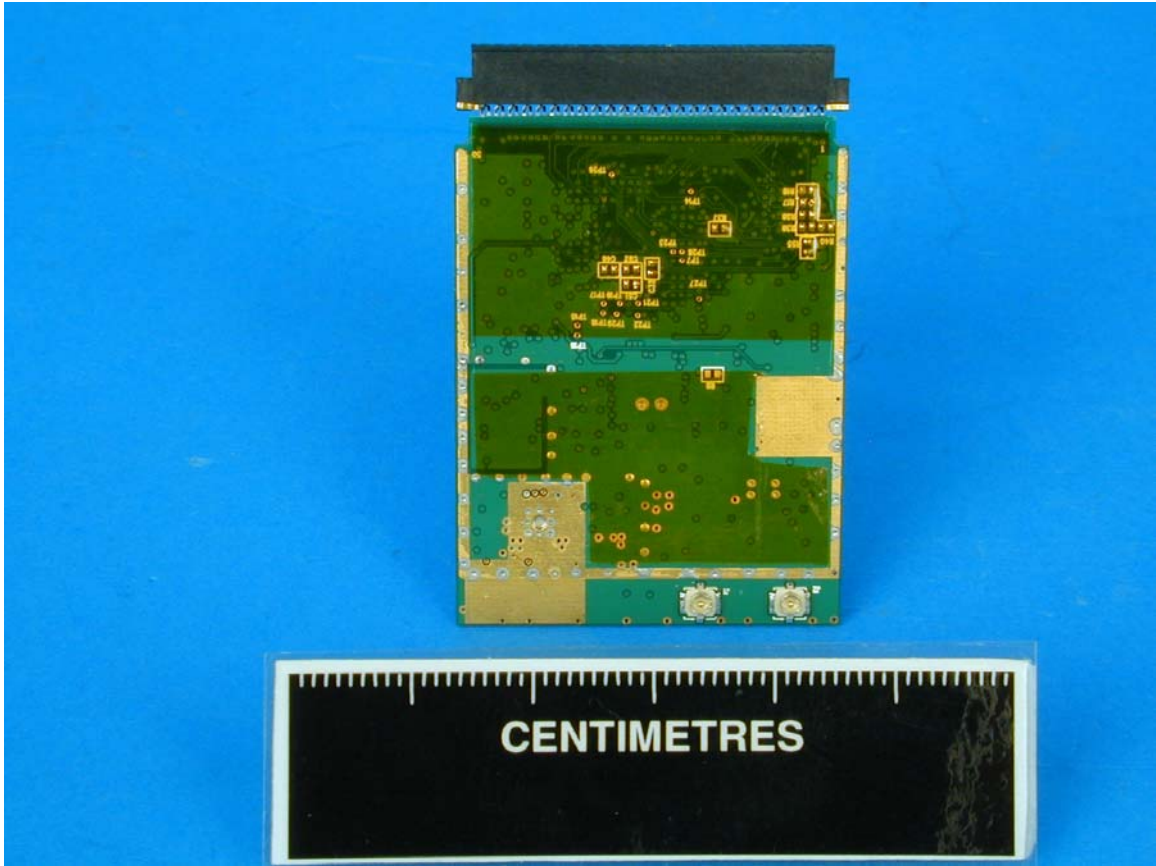
Bottom view shielding removed, 802.11b radio module
