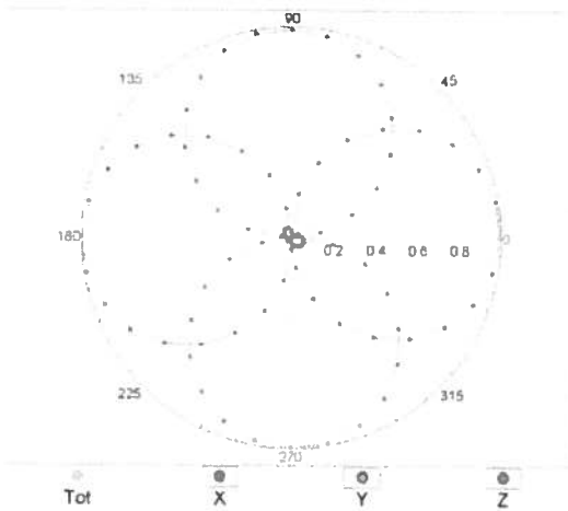
f=600 MHz,TEM,0°
