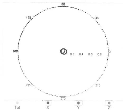
f=2500 MHz,R22,90°
