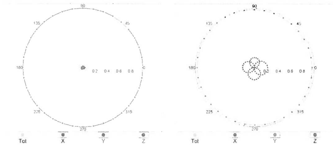
f=600 MHz, TEM, 90^\circ
