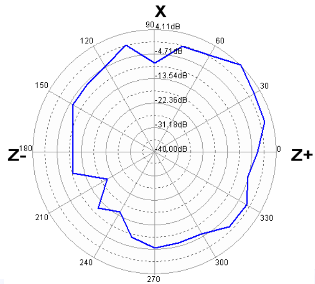
Passive Test E-Total (X-Z Plane)
