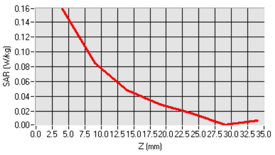
SAR, Z Axis Scan (X = 25, Y = -16)
