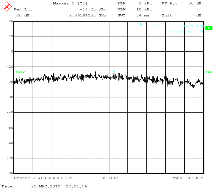
PSD High Channel (802.11n-20MHz-2.4G)
