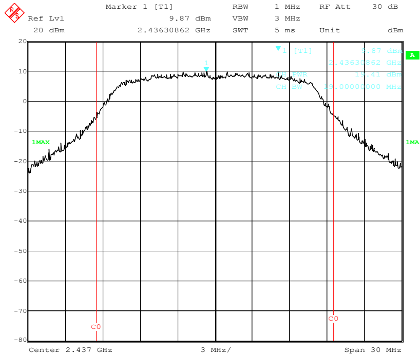
Output Power Middle Channel (802.11g)
