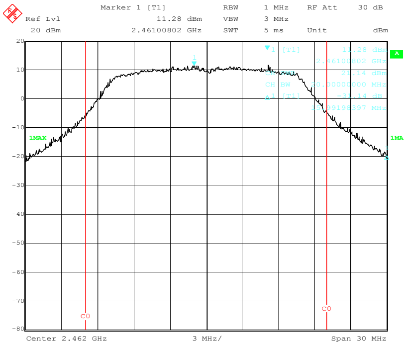
Output Power High Channel (802.11g)
