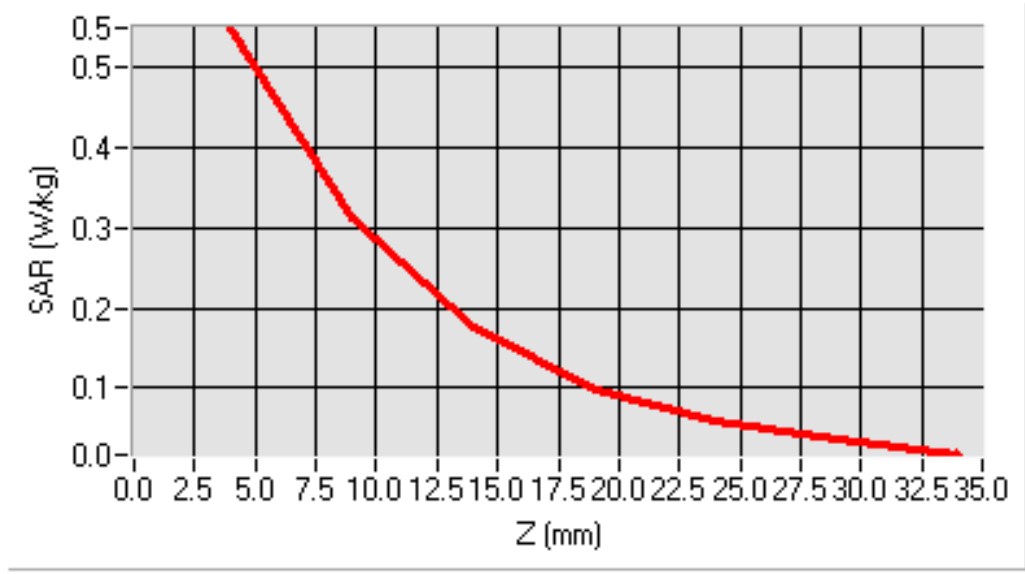
SAR, Z Axis Scan (X = -2, Y = -6)
