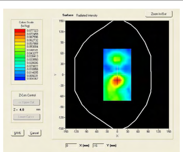
SAR, Z Axis Scan (X = 0, Y = -16)
