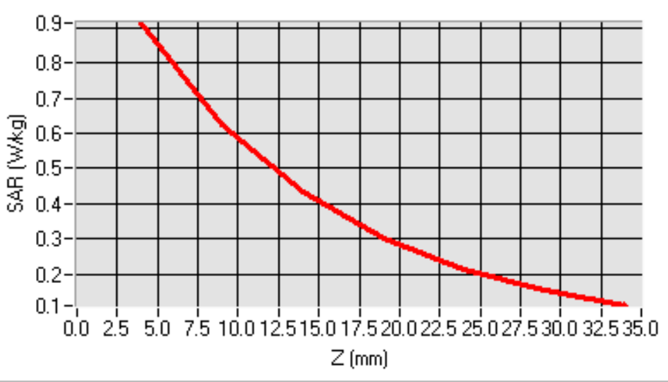
SAR, Z Axis Scan (X = 0, Y = 1)
