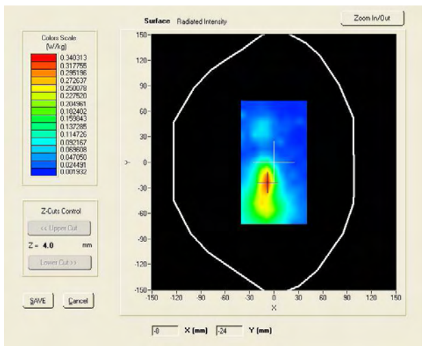
SAR, Z Axis Scan (X = -8, Y = -24)
