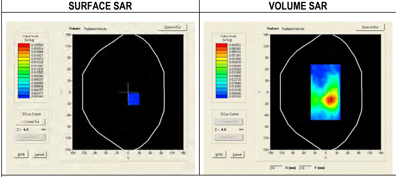
SAR, Z Axis Scan (X = 15, Y = -18)
