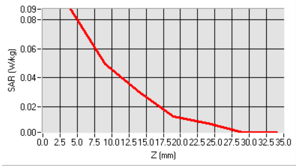
SAR, Z Axis Scan (X = 0, Y = -16)
