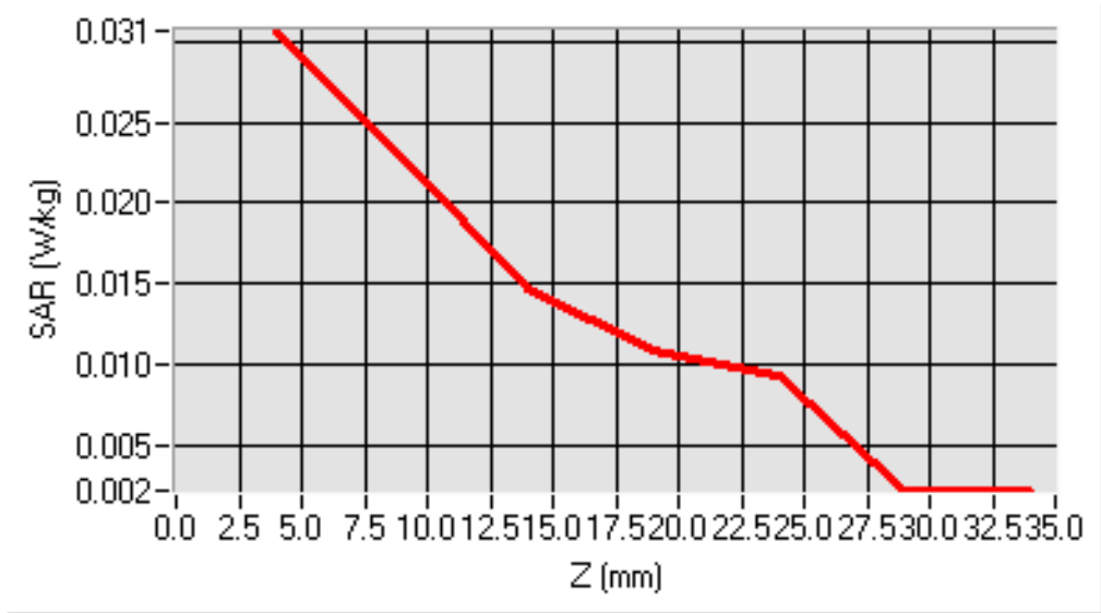
SAR, Z Axis Scan (X = 40, Y = -8)
