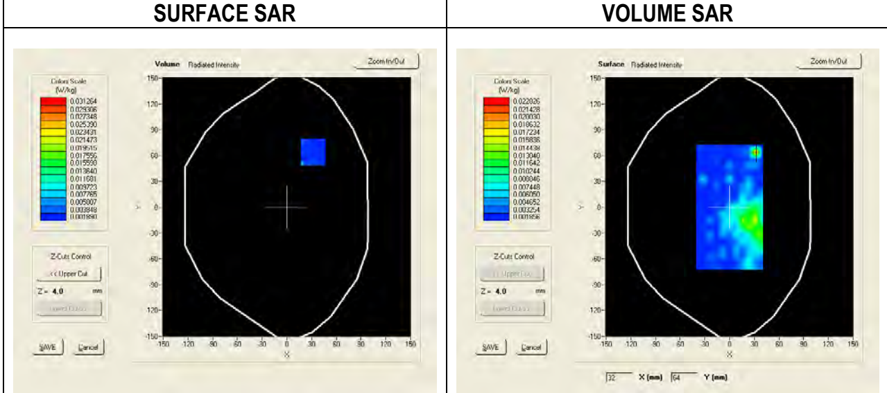
SAR, Z Axis Scan (X = 32, Y = 64)
