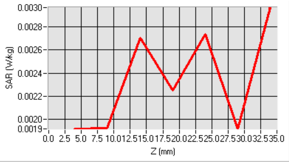
SAR, Z Axis Scan (X = 15, Y = -18)
