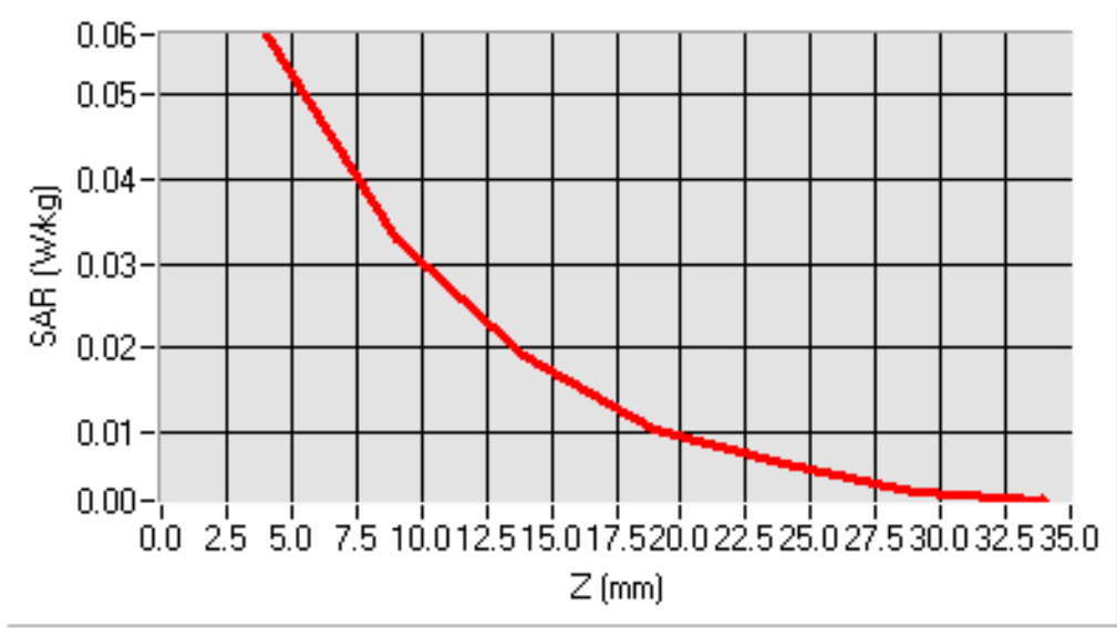
SAR, Z Axis Scan (X = 26, Y = 5)
