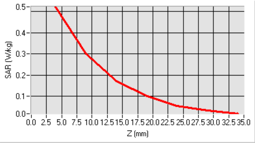
SAR, Z Axis Scan (X = -2, Y = -6)
